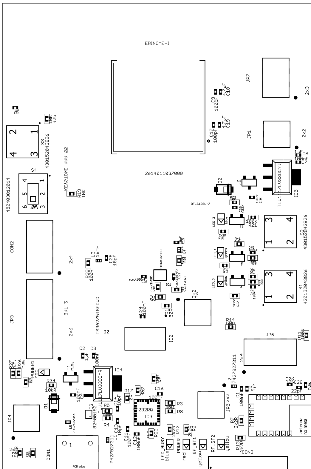
Figure 10: Assembly diagram
