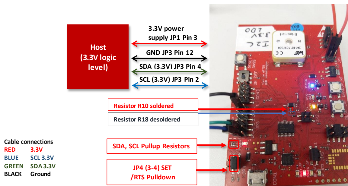
Figure 16: Erinome-I evaluation board connection to 3.3 V Host
