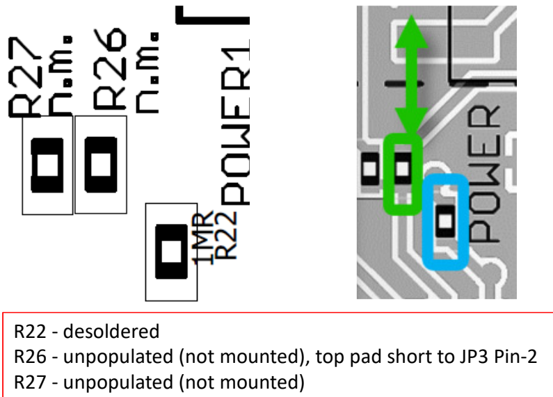
Figure 19: R22, R66 and R27 after SPI modifications
