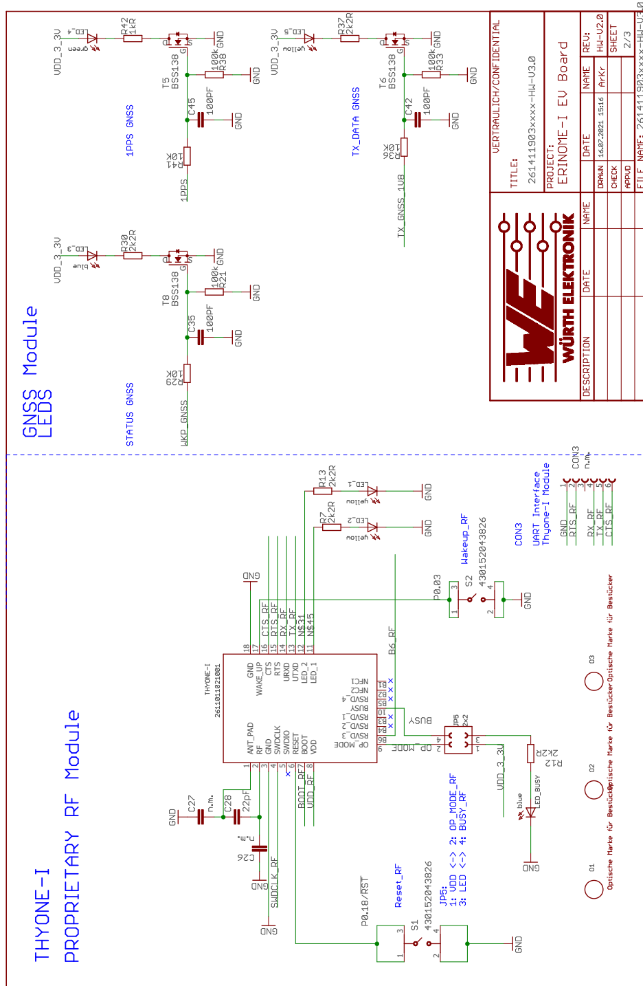
Figure 8: Schematic sheet-2
