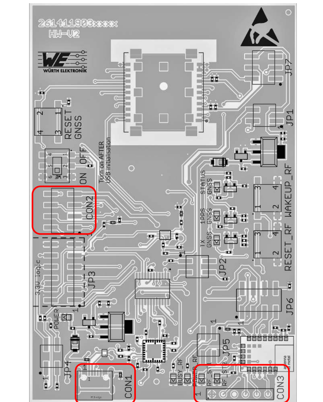
Figure 5: Connectors
