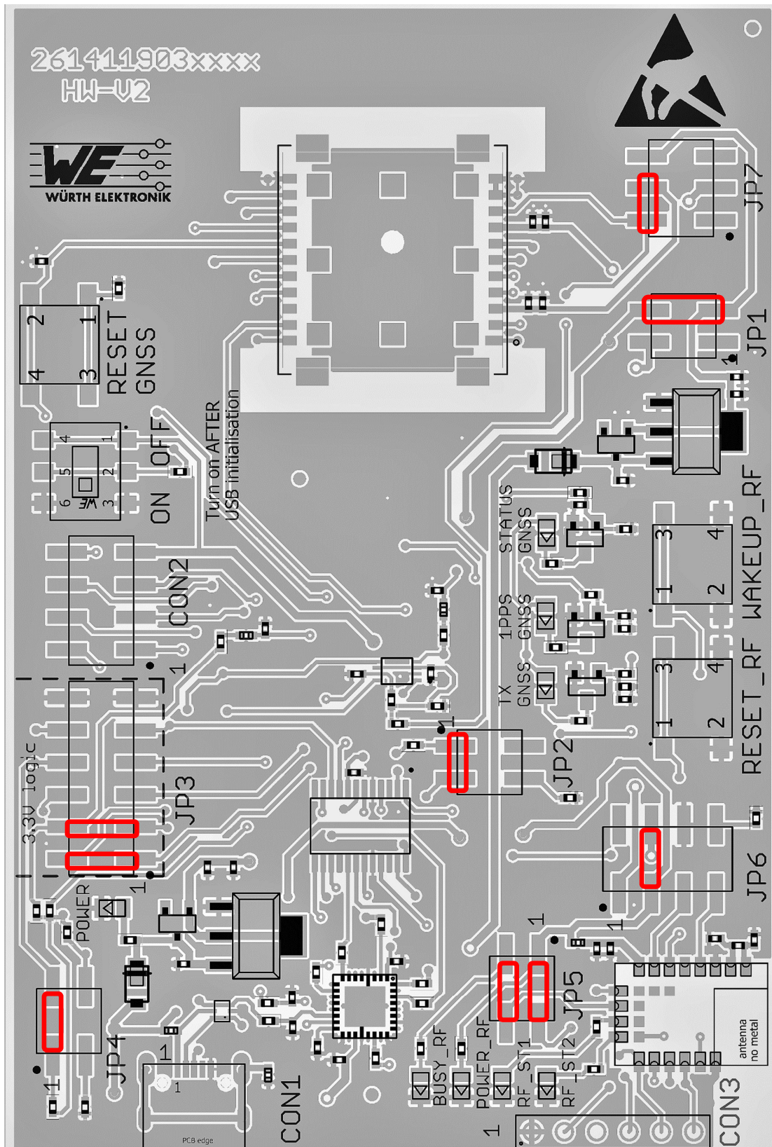
Figure 4: Jumpers - default setting
