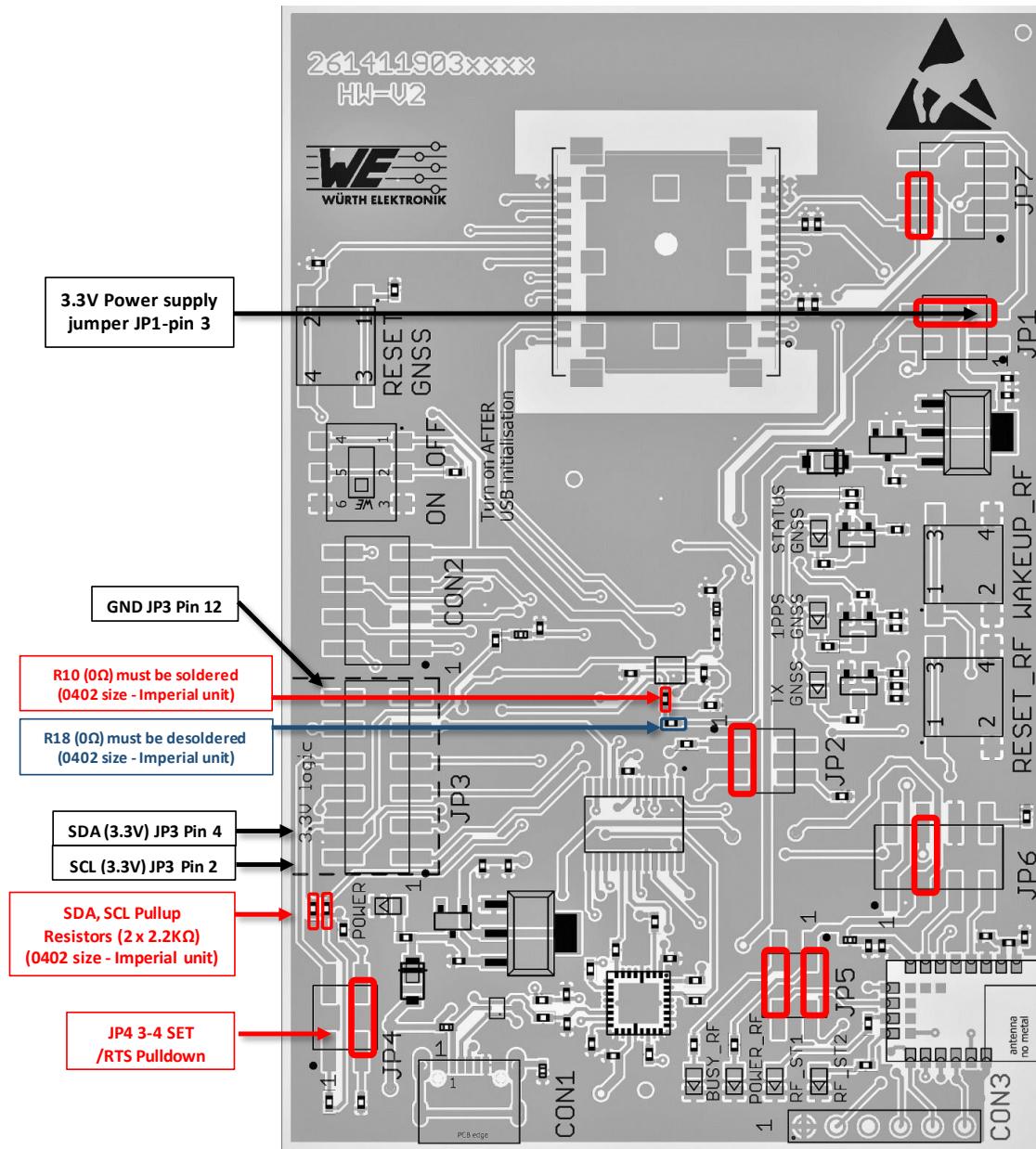
Figure 15: I 2 C evaluation board modification - Erinome-I
